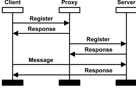
Figure 5. An MSC containing a race condition.
