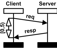
Figure 2. MSC with time.
