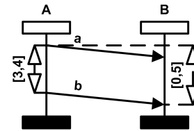
Figure 4. An MSC with a too wide time interval.
