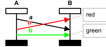
Figure 7. The output of the Find Flow function for the MSCs depicted in Figure ???. Red message should be removed and the green one should be added in Flow to match Spec .
