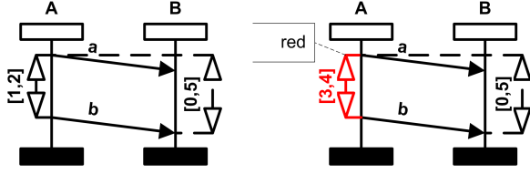
Figure 8. The BMSC on the right is returned when the Find Flow function searches the BMSC on the left in the BMSC of Figure ???. The problematic time interval [3, 4] is highlighted in red.
