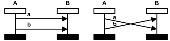
Figure 6. An MSC Spec (left) and an MSC Flow (right).
