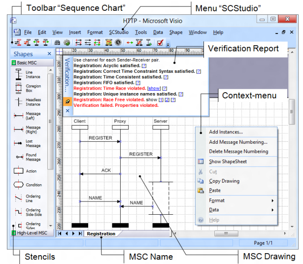
Figure 3. Screenshot of MS Visio with the SCStudio add-on.
