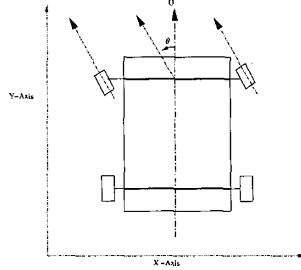
Fig. 1. Robot Model
