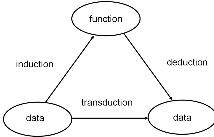
Figure 1.1 The relations among induction, deduction and transduction.
