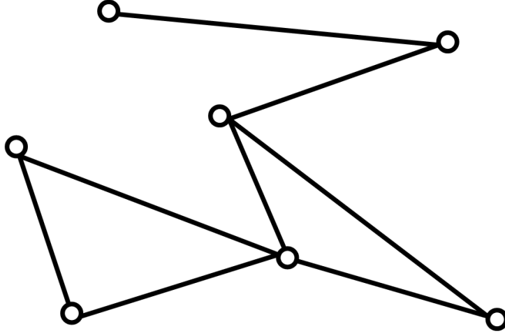
Figure 1.2 An undirected graph.
