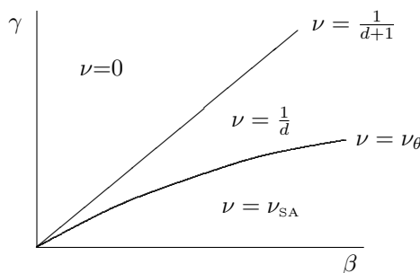
Figure 1: Sketch of the conjectured values for \nu(\gamma, \beta) .
