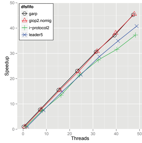
(b) DFS_FIFO
