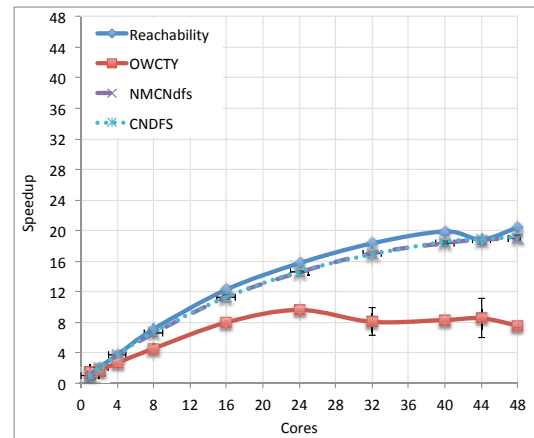
Figure 7.6: Speedup synapse.7.p3
