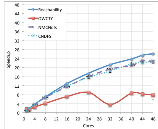
Figure 7.2: Speedup bobp.4.p3
