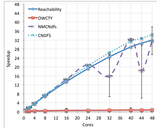
Figure 7.4: Speedup ldrflt.6.p2
