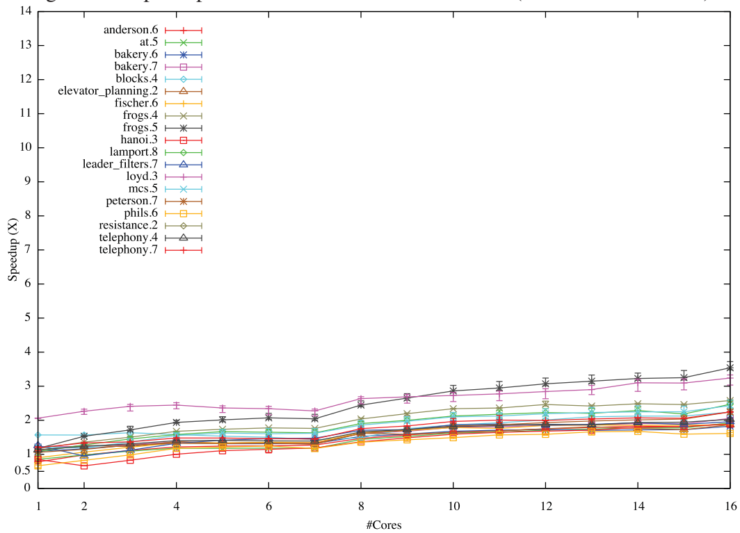
Figure 2.4: Speedup of BEEB models with DiViNE 2.2 (DiViNE as base case)
