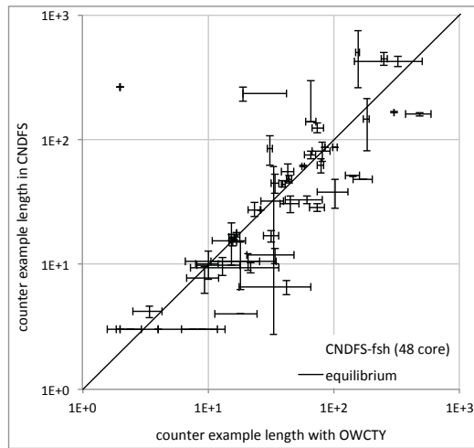
Figure 7.9: Fsh vs OTF_OWCTY (48 cores)
