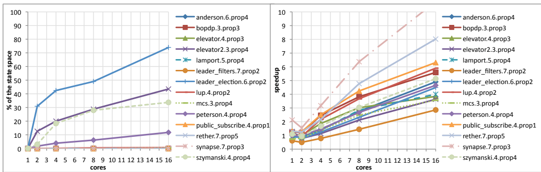
Figure 6.11: Cumulative extra work due to NMC-NDFS repair.
