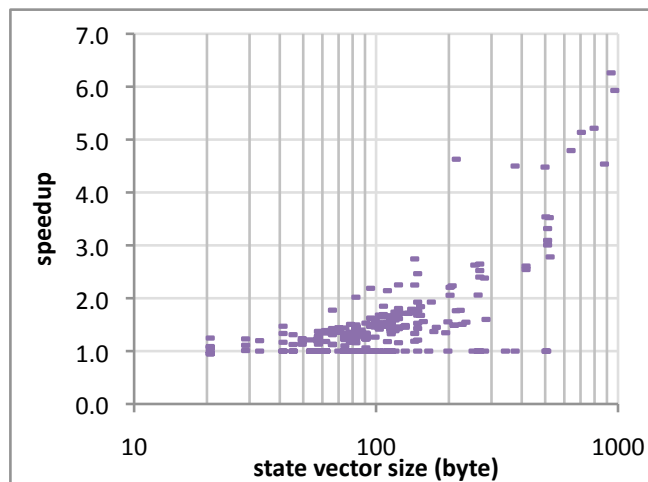
Figure 3.10: Speedup of Algorithm 3.8 wrt. Algorithm 3.4.
