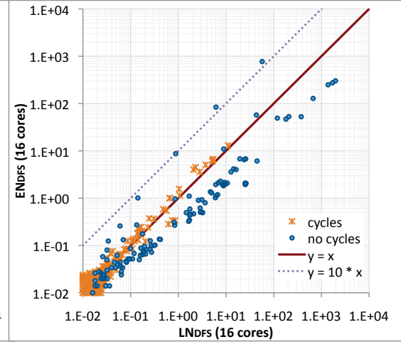
Figure 6.10: ENDFS vs LNDFS.
