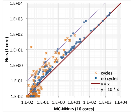
Figure 5.5: Log-log scatter plot of MC-NDFS/ multi-core SV NDFS run-times.
