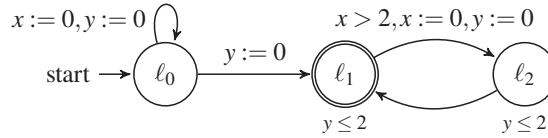
Figure 10.1: A timed Büchi automaton.
