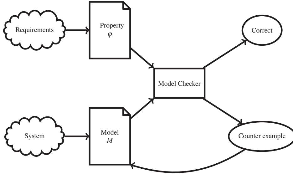
Figure 1.2: The workflow in modelchecking
