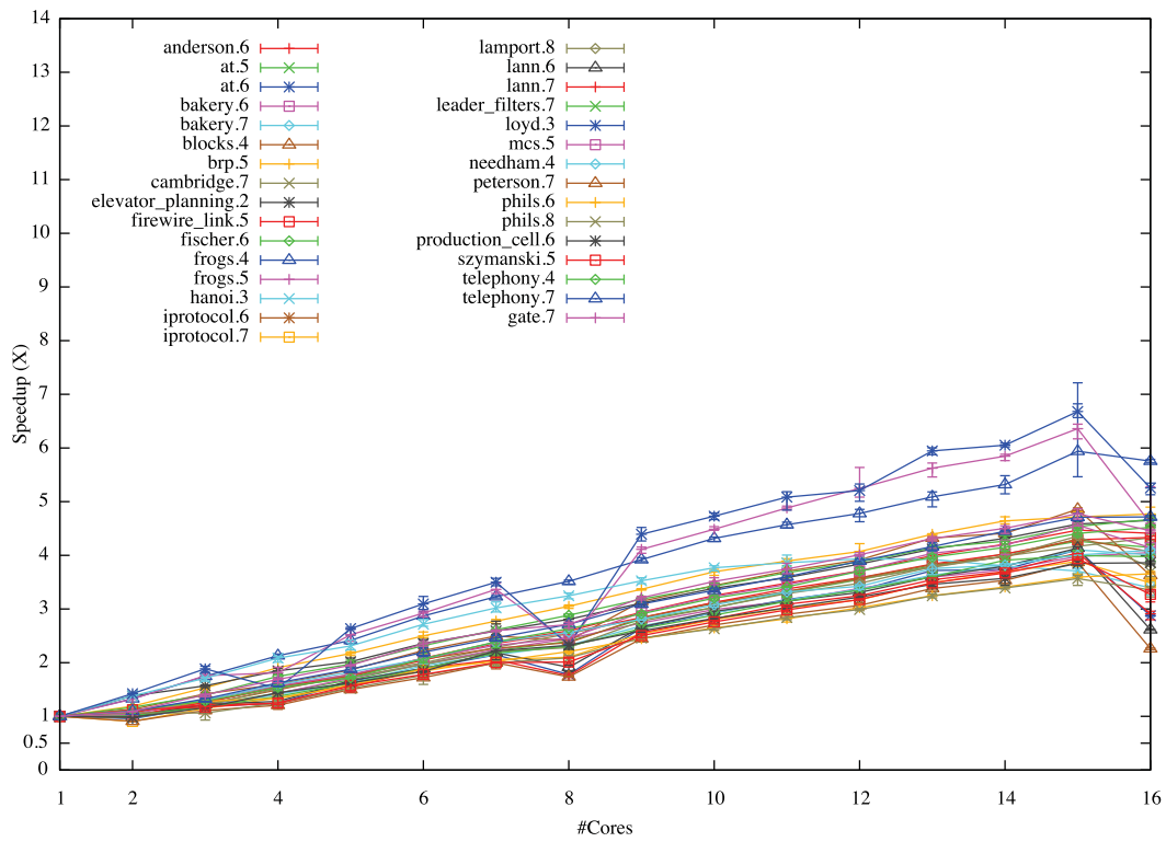
Figure 2.4: Speedup of BEEB models with DiViNE 2.2 (DiViNE as base case)
