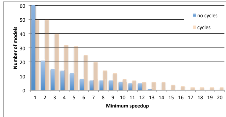
Figure 5.6: Model counts of speedups with MC-NDFS (base case: sequential NDFS)
