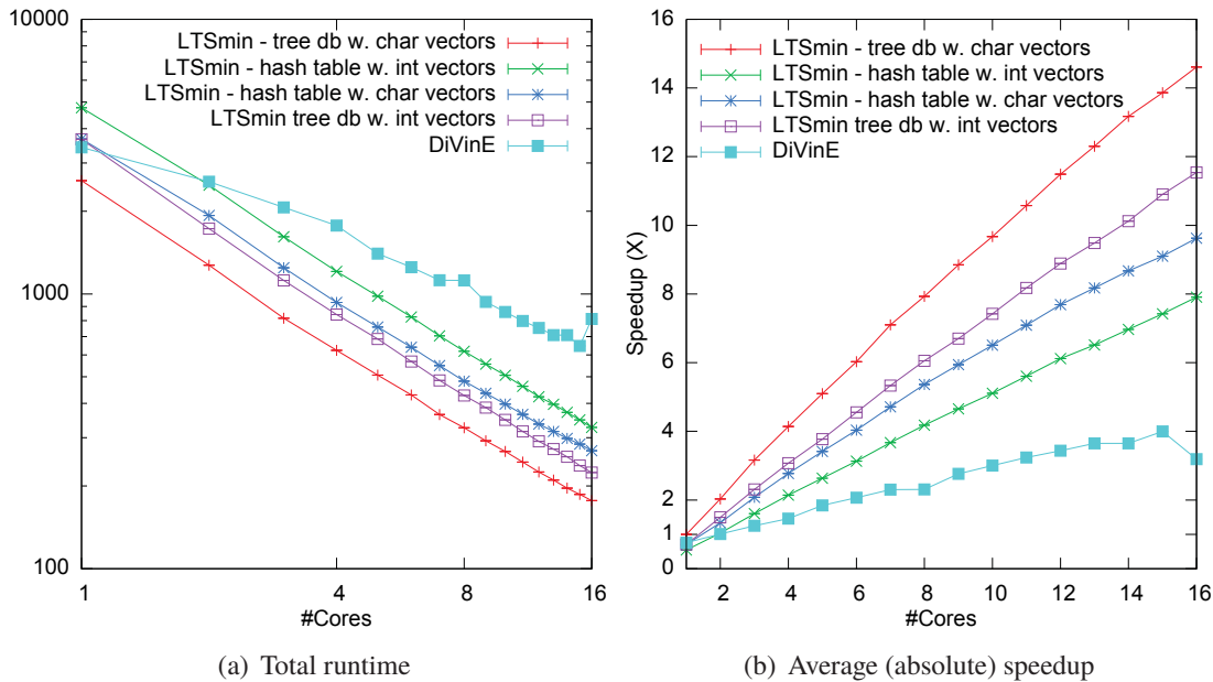
Figure 3.17: Performance benchmarks for 158 models with \text{DiVINE} (hash table) and with \text{LTS}_{\text{MIN}} using tree compression and hash table.
