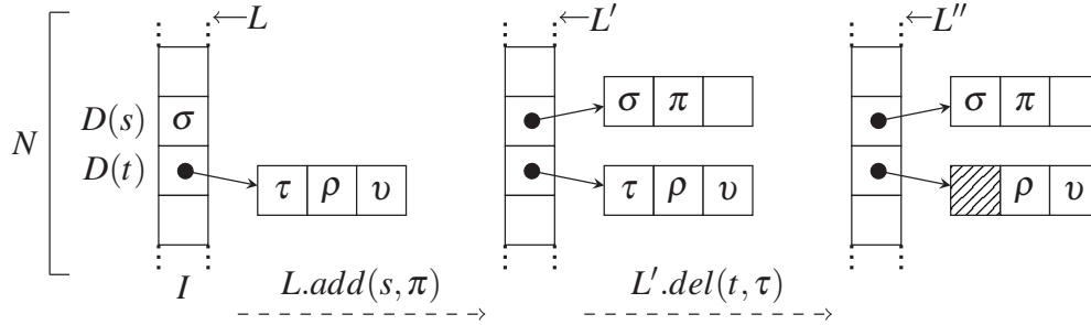
Figure 9.2: Data structure for L , and operations
