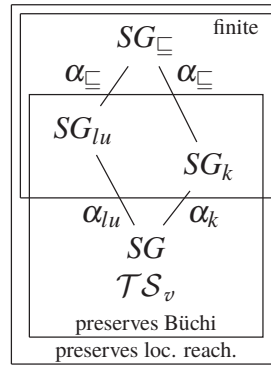
Figure 10.3: Abstractions.
