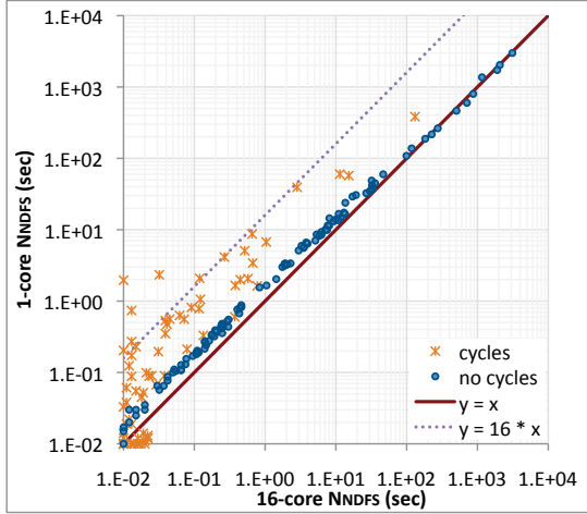
Figure 5.4: Log-log scatter plot of multi-core SV NDFS/ sequential NDFS run-times.
