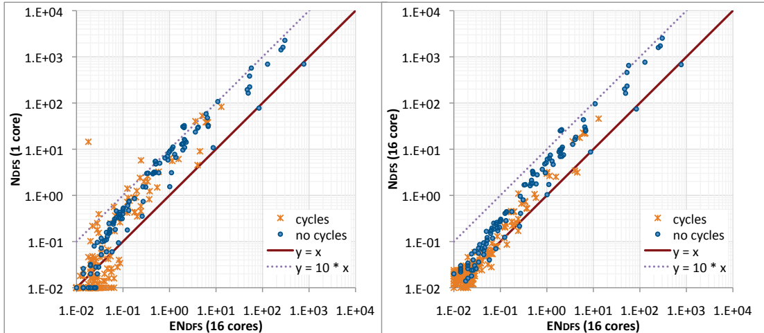
Figure 6.3: N_{DFS} vs EN_{DFS} .
