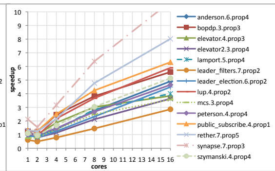
Figure 6.12: Speedups OwCTY.
