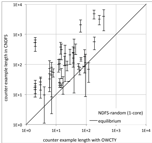
Figure 7.8: NDfs vs OTF_OWCTY (1 core)
