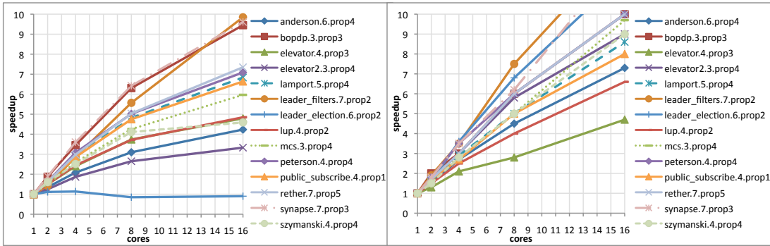
Figure 6.1: Measured speedups ENDFS.
