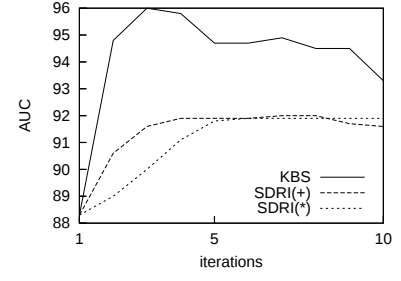
Figure 4: Ionosphere
