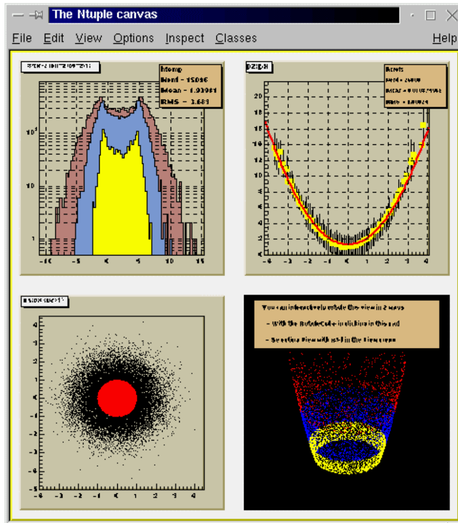
Figure 4: ROOT Histograms
