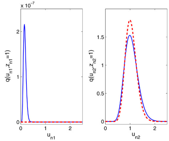
Fig. 7. The typical joint variational posterior q(\mathbf{u}_n | \mathbf{z}_n) of the indicator and the scale variable for a single data point \mathbf{x}_n . The mixture has two components. The data is the Old Faithful Geyser data. The solid curve does not neglect the correlation between both latent variables (type-2 SMM), while the dashed curve does (type-1 SMM).
