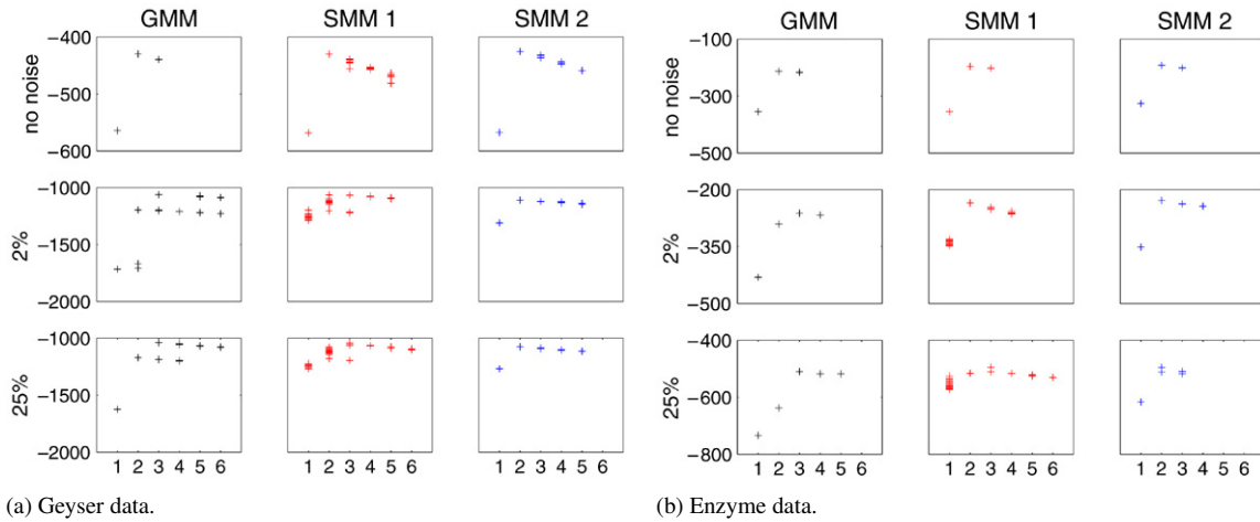
Fig. 4. Variational lower bound for (a) the Old Faithful Geyser data and (b) the Enzyme data versus the number of components. An increasing number of outliers is successively added to the training set. Results are reported for the Bayesian GMM, as well as the type-1 and type-2 Bayesian SMM. Twenty runs are considered for all model complexities. The value of the bound obtained for each run is indicated by a cross. It is important to realize that the number of crosses for each model complexity might differ from method to method. The reason is that mixture components are pruned out during the learning process when there is too little evidence for them. Therefore, we did not use a standard representation such as box and whiskers plots to show the variability of the results but preferred this more intuitive representation.
