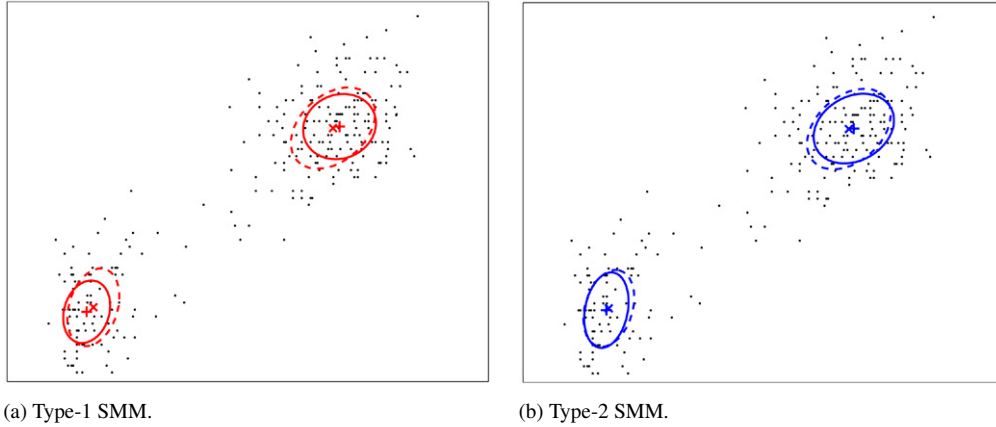
Fig. 6. Old Faithful Geyser data. The markers 'x' and '+' indicate respectively the means in absence and presence of outliers (25%). The dashed curves and the solid curves correspond respectively to single standard deviation in absence and presence of outliers. The models are constructed with two components.
