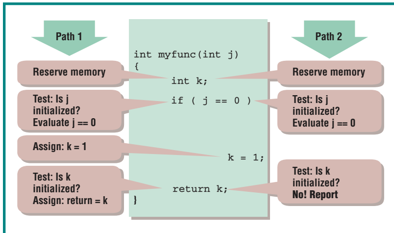
Figure 1. The PREFIX tool. PREFIX traces two paths through this function, produces a model, and analyzes it for errors.
