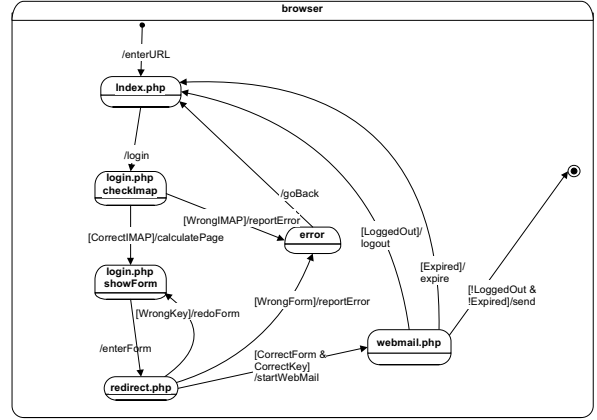
Figure 9. Top-level statechart of the browser
