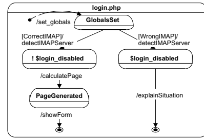
Figure 8. Refactoring on the initial statechart in Figure 7
