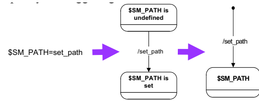
Figure 4. Statechart notations
