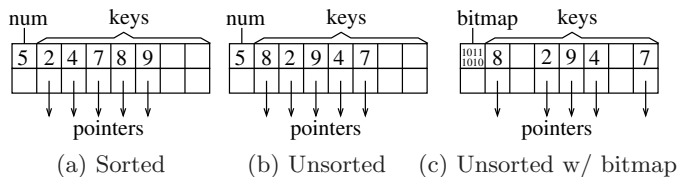
Figure 3: B + -tree node organizations.
