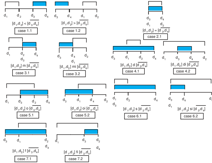
Fig. 4. Allen's intervals for [d_1, d_2]([d_3, d_4])p
