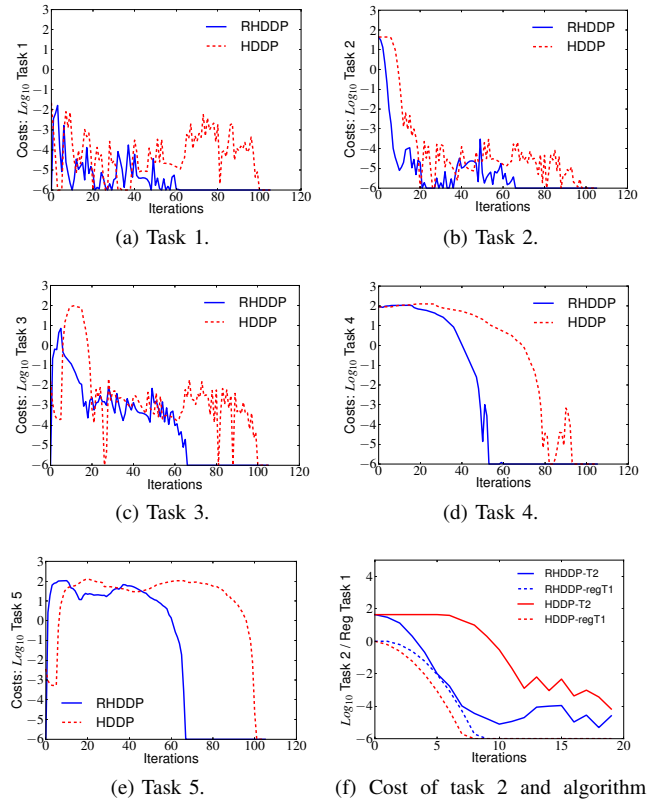
Fig. 11. Test 4: convergence of the cost functions using the algorithm presented in this paper (RHDDP) and its previous version (HDDP [10]).
