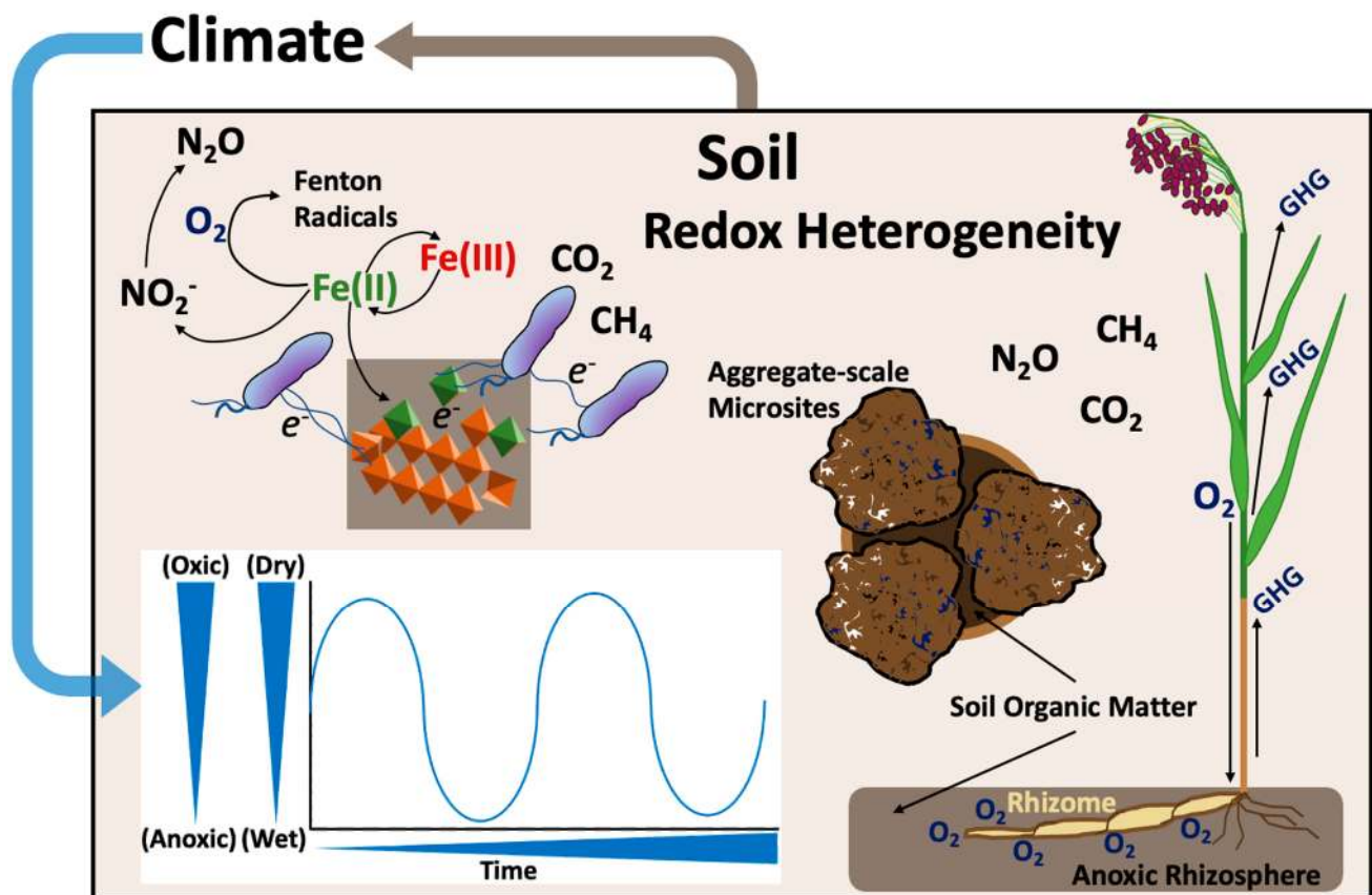
Figure 1. Conceptual framework of fine-scale redox heterogeneity in soils. The framework illustrates redox heterogeneity spanning mineral, microbial, organic, aggregate, and wetland–rhizosphere interfaces. Greenhouse gases ( \text{CH}_4 , \text{CO}_2 , \text{N}_2\text{O} , GHGs) are shown in different pathways. The blue oscillation graph in the lower left corner indicates soil conditions that vary with time and correlate with redox heterogeneity relevant to all the scenarios shown in the main figure. The large brown and blue arrows revolving in the upper left corner indicate soil and climate interactions. Between the head of the blue arrow and the tail of the brown arrow, these interactions are entangled by redox heterogeneity. The mineral, microbial, organic, aggregate, and wetland–rhizosphere features, as well as the oscillating conditions, can be envisioned to coexist in different environmental systems discussed in the main text and are not meant to be mutually exclusive in this framework. Additionally, though not explicitly shown, other organisms such as earthworms and various soil mesofauna collectively form an integral part of this conceptual framework, especially because they transfer and transform soil organic matter, influence aggregate structure, degrade plant tissues, and open physical channels for nutrient and gas exchange among the different soil interfaces.
