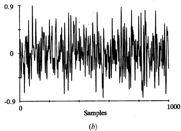
Figure 9. System outputs and inputs (Example 2): (a) outputs y(t) ; (b) inputs u(t) .
