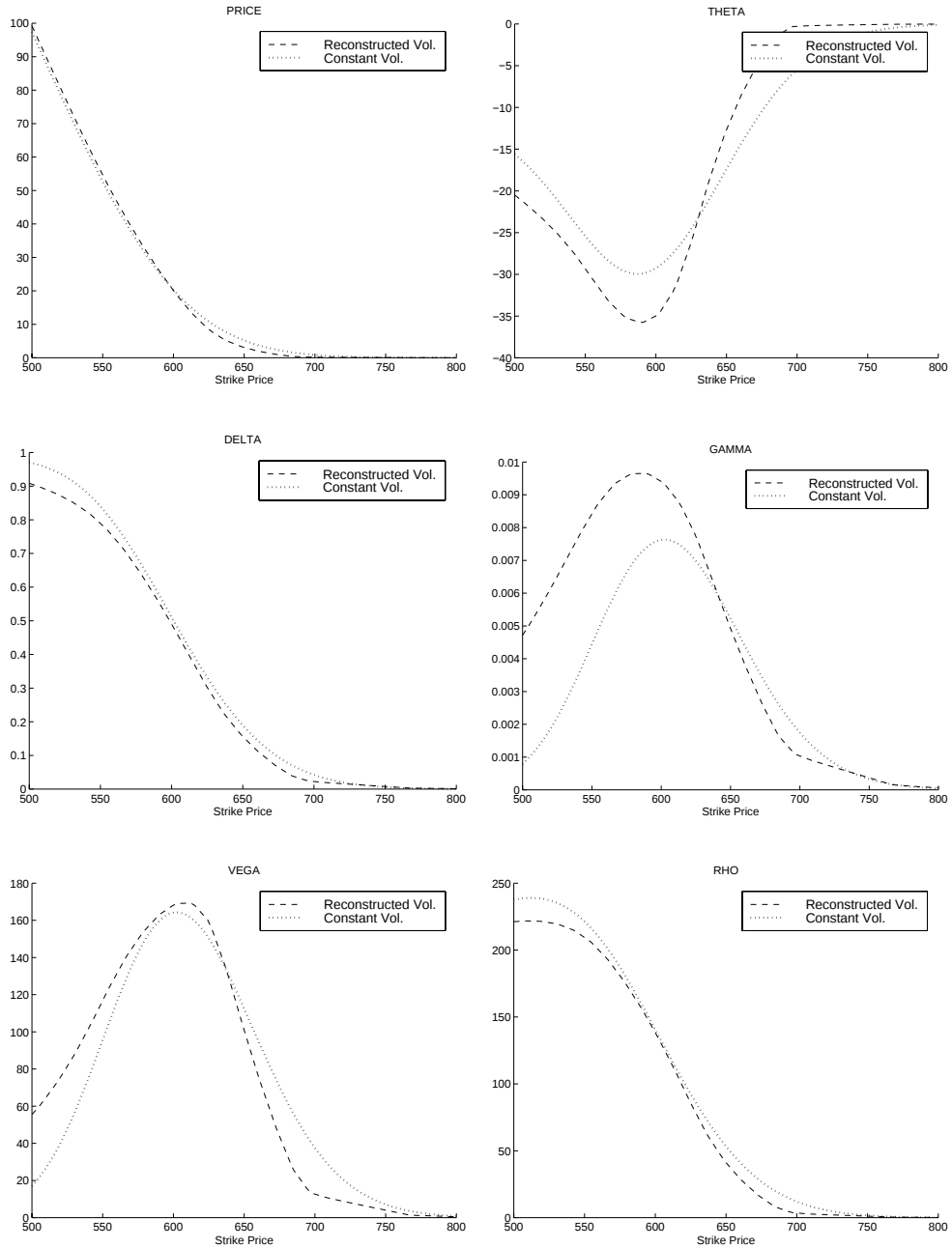
FIG. 8. Comparison Using the Reconstructed Versus Constant (average) Volatility
