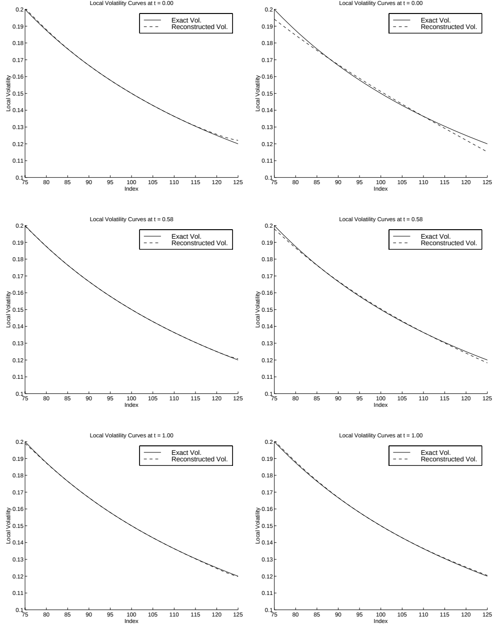
FIG. 3. Left: Knots = [0 : .2S_{init} : 2S_{init}] \times [0, 1] , Right: Knots = [.4S_{init} : .4S_{init} : 1.6S_{init}] \times [0, 1]
