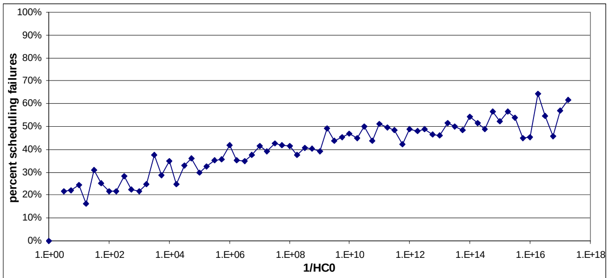
Figure 14: RM scheduler with preemption, percentage of scheduling failures per 1/HCO
