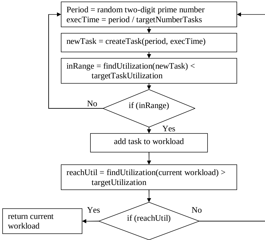
Figure 4: Process for generating workloads, method 3
