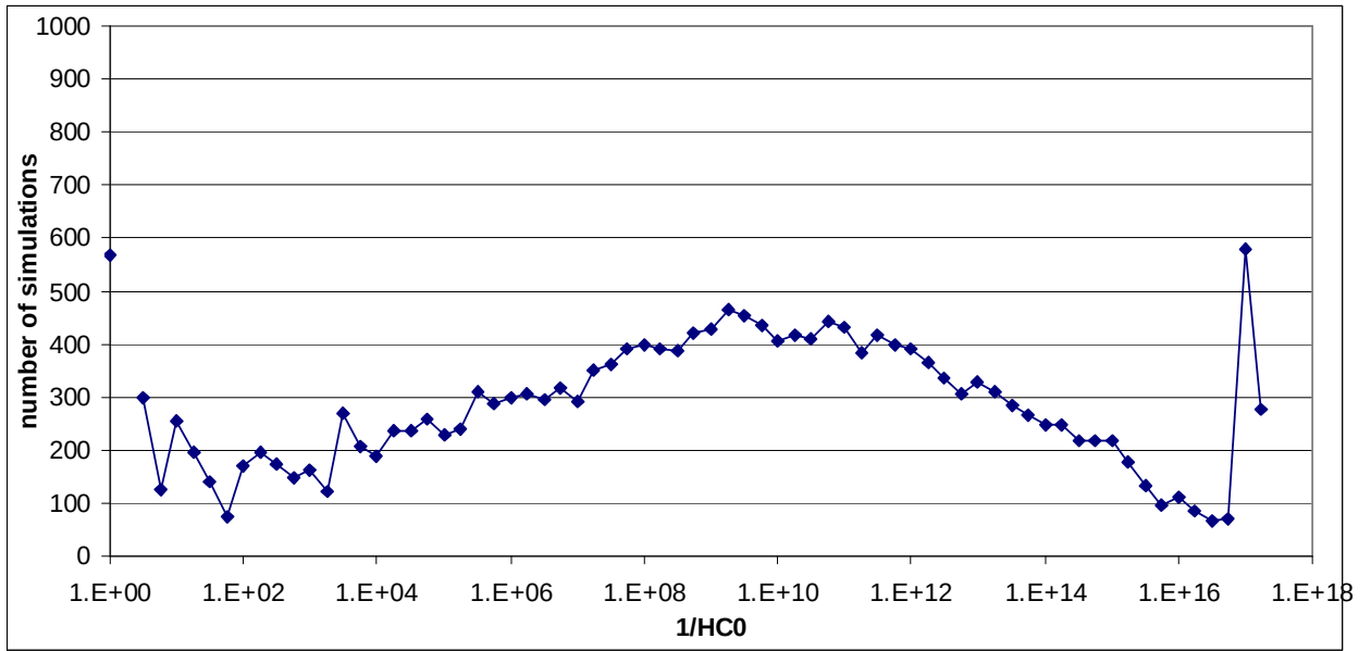
Figure 13: RM scheduler with preemption, simulations per 1/HCO
