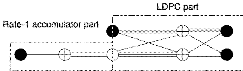
FIG. 2 (Prior Art)
