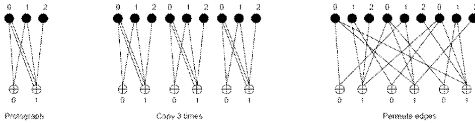
FIG. 1 (Prior Art)
