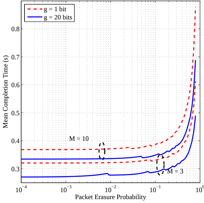
Fig. 7. Mean completion time for the TDD scheme with two receivers with different M and field sizes q = 2 and q = 1048576 , for g = 1 and g = 20 bits, respectively. We use the following parameters R = 1.5 Mbps, h = 80 bits, n_{ack} = 100 bits.
