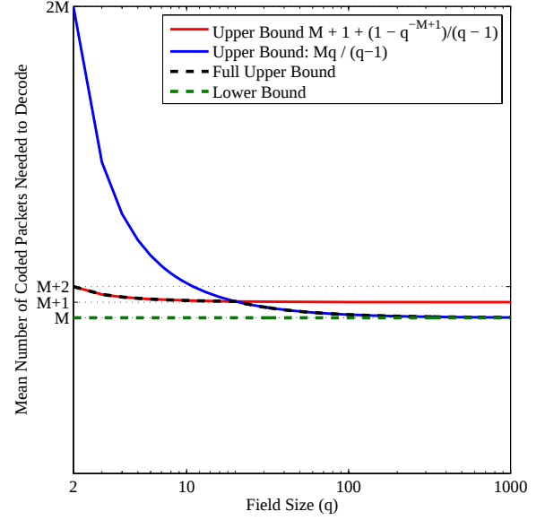
Fig. 3. Upper and Lower bounds on the mean number of coded packets needed at the receiver in order to decode versus the field size q .
