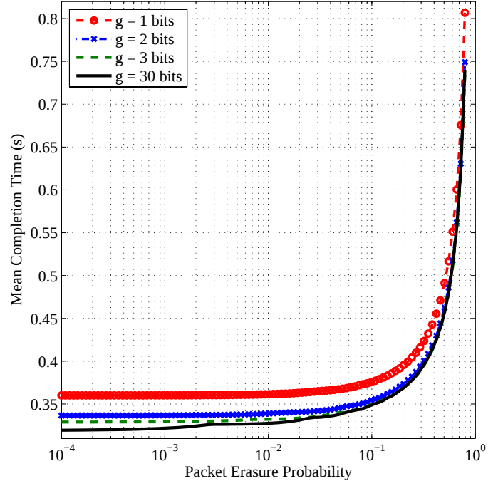
Fig. 6. Mean completion time for the TDD scheme with a single receiver with different field sizes q = 2^g . We use the following parameters R = 1.5 Mbps, h = 80 bits, n_{ack} = 100 bits, M = 10 .
