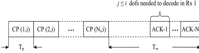
Fig. 4. [4] Network coding TDD scheme for broadcast.
