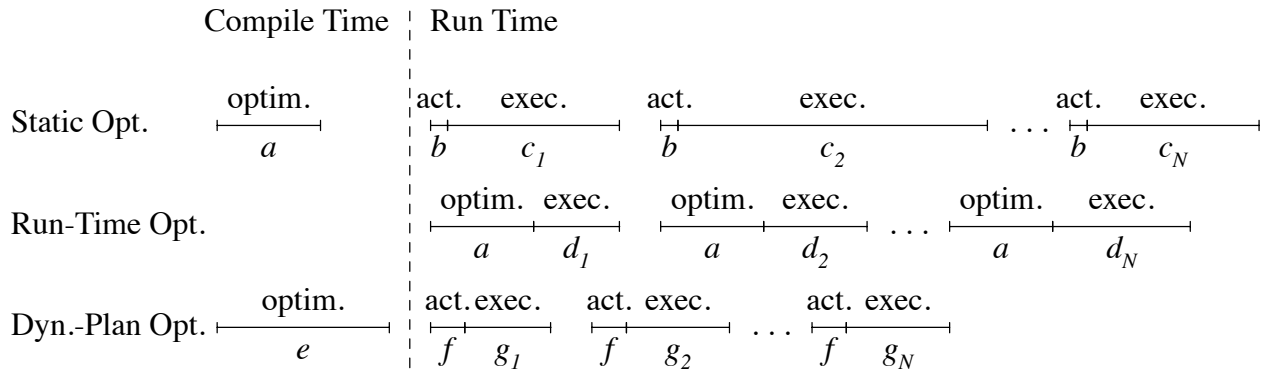
Figure 45. Optimization Options for Queries with Run-Time Bindings.
