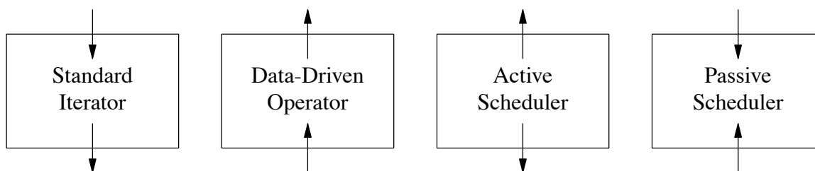
Figure 43. Operators, Schedulers, and Control Flow.
