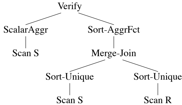
Figure 19. Query Plan for Division by Sort-Based Aggregation.
