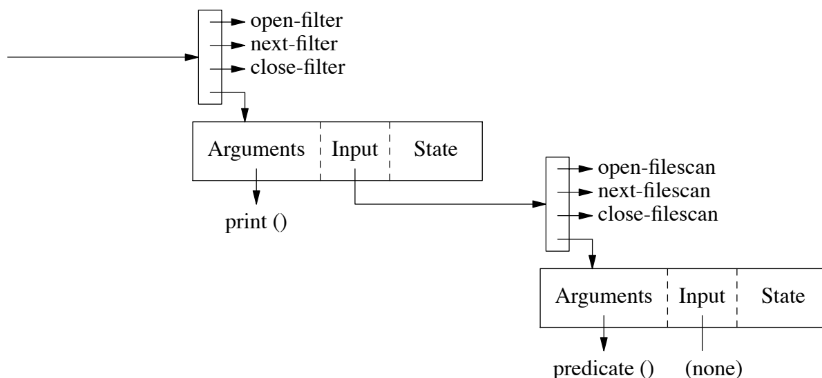
Figure 5. Two Operators in a Volcano Query Plan.
