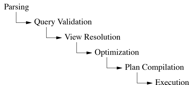
Figure 2. Query Processing Steps.
