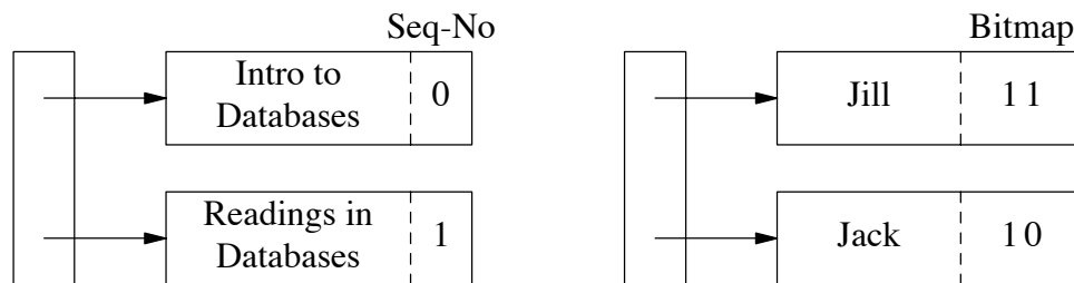
Figure 21. Divisor Table and Quotient Table in Hash-Division.
