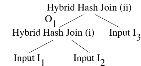
Figure 28. Plan for Joining Three Inputs.
