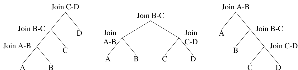
Figure 4. Left-Deep, Bushy, and Right-Deep Plans.
