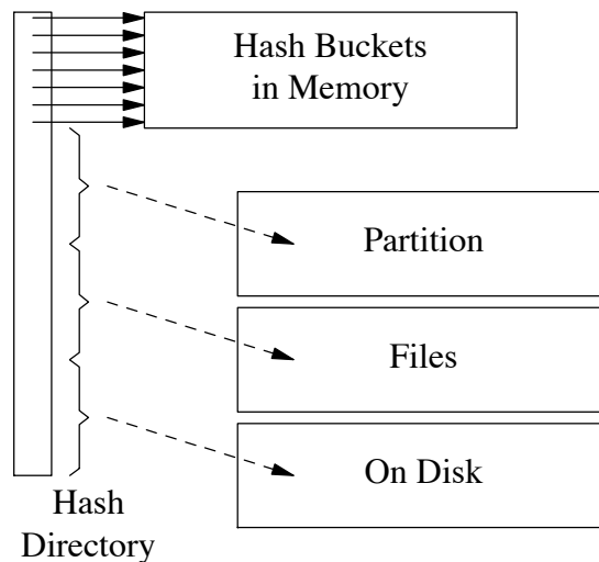
Figure 9. Hybrid Hashing.
