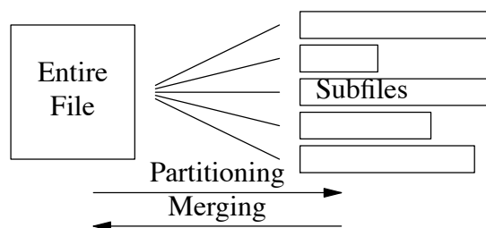
Figure 23. Partitioning Skew.
