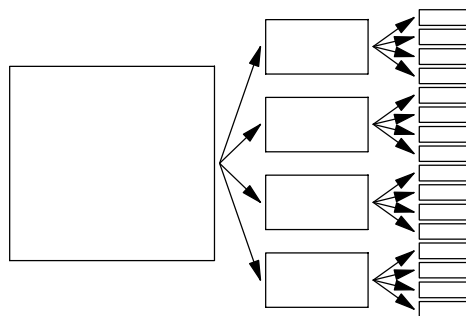
Figure 10. Recursive Partitioning.
