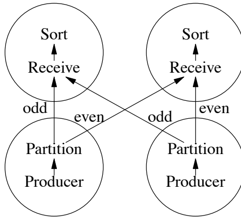
Figure 38. Deadlock-Free Scenario.
