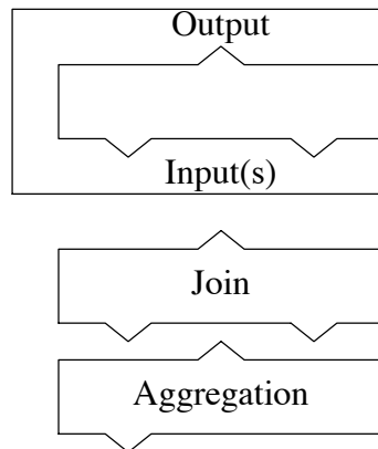
Figure 31. Bracket Model of Parallelization.
