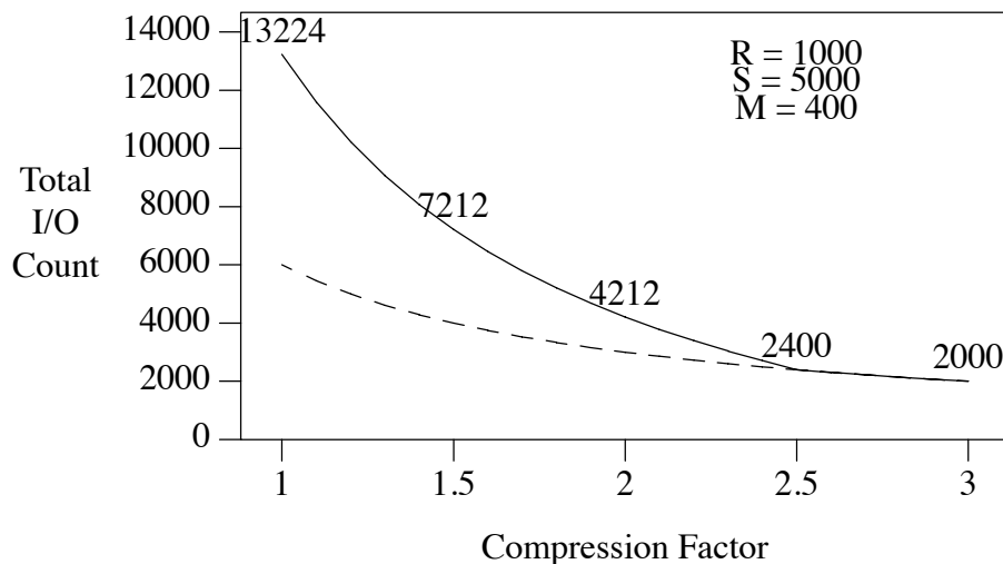
Figure 44. Effect of Compression on Hybrid Hash Join Performance.
