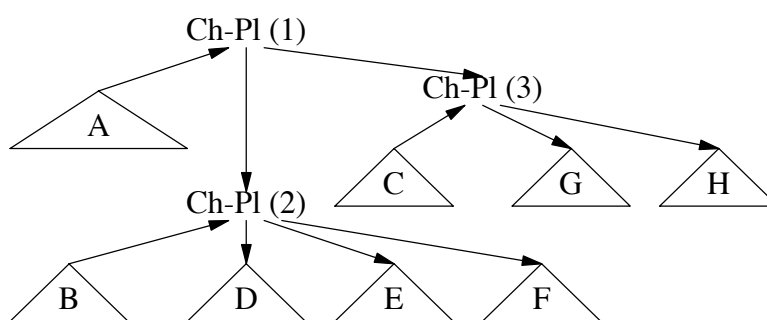
Figure 30. Implementation using Choose-Plan Operators.
