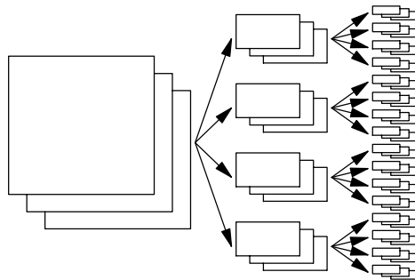
Figure 26. Partitioning in a Multi-Input Hash Join.
