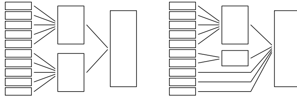
Figure 6. Naive and Optimized Merging.
