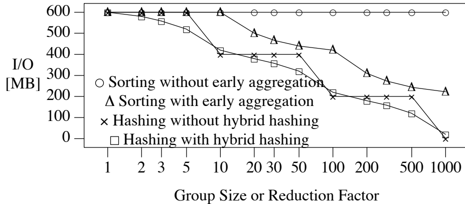
Figure 14. Performance of Sort- and Hash-Based Aggregation.
