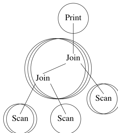
Figure 33. Processes Created by Exchange Operators.
