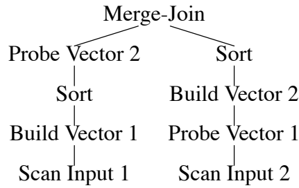
Figure 24. Merge-Join with Symmetric Bit Vector Filtering.
