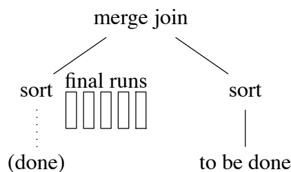
Figure 27. The Stop Point During Sorting.
