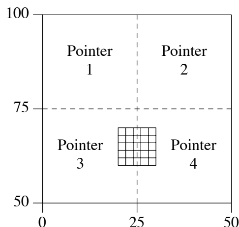
Figure 11. A Node in a Quadtree.
