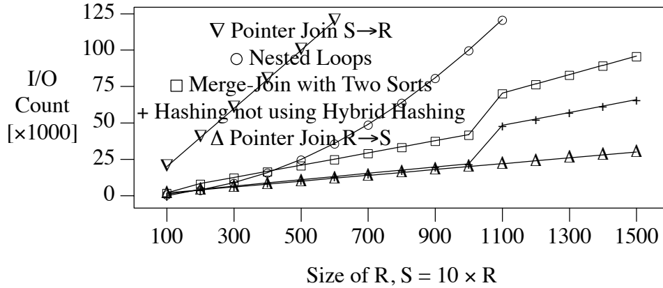
Figure 18. Performance of Alternative Join Methods.
