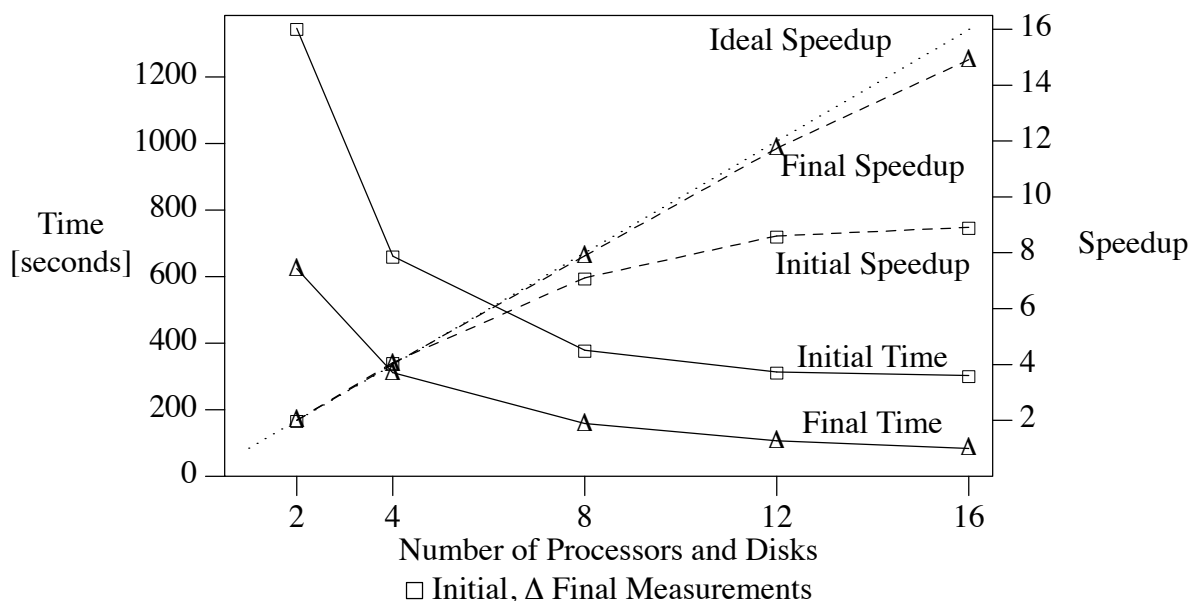
Figure 35. Tuning Effectiveness for a Parallel Algorithm.
