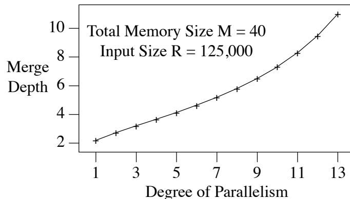
Figure 40. Merge Depth as a Function of Parallelism.
