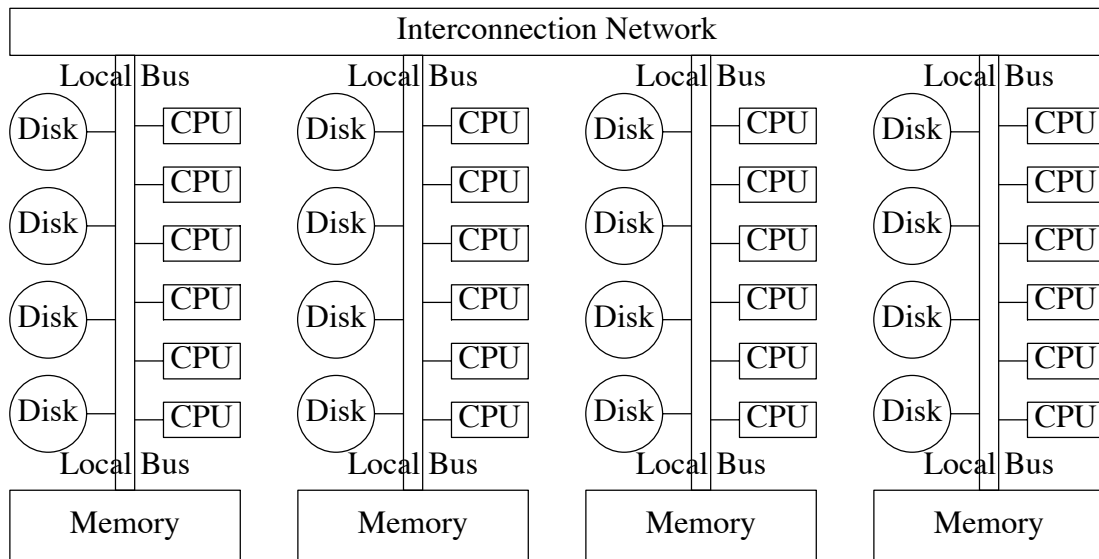
Figure 36. A Hierarchical-Memory Architecture.
