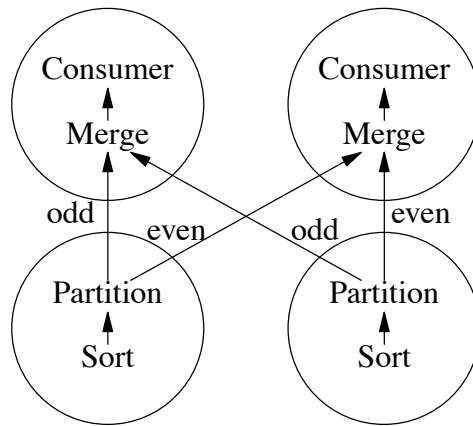
Figure 37. Scenario with Possible Deadlock.
