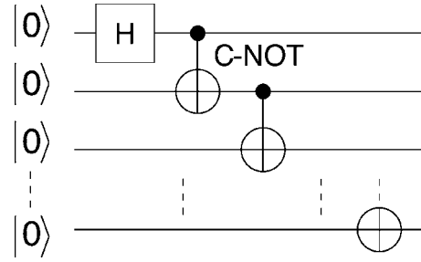
FIG. 1. Quantum circuit for generating the N -qubit Greenberger-Horne-Zeilinger (GHZ) state. The gates (unitary transformations) are a Hadamard gate (“ H ”) and pairwise-acting controlled-NOT gates.
