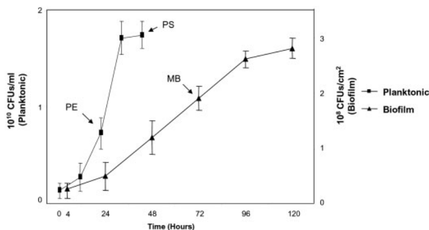
Figure 1. Growth kinetics of planktonic and biofilm B. pertussis Tohamal cells in Stainer–Scholte medium at 37°C. Planktonic cells (■) were harvested from Erlenmeyer flasks, whereas sessile cells (▲) were recovered from flat polypropylene beads of a glass column bio-reactor. Arrows indicate the harvesting point for FT-IR spectroscopy and proteomic analysis. Results are averages of at least three independent experiments. PE: planktonic cells in exponential phase; PS: planktonic cells in stationary phase and MB: cells in mature biofilm.
