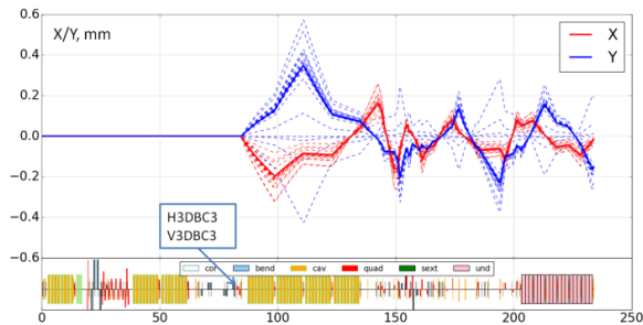
Figure 3: Orbits changing during Action1 .
