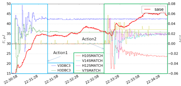
Figure 2: SASE optimization at \lambda=13.5 nm.
