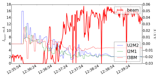
Figure 6: Injection tuning.
