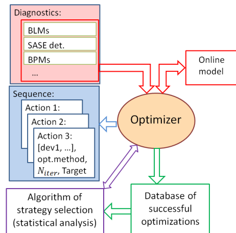
Figure 1: Scheme of the optimization tool.
