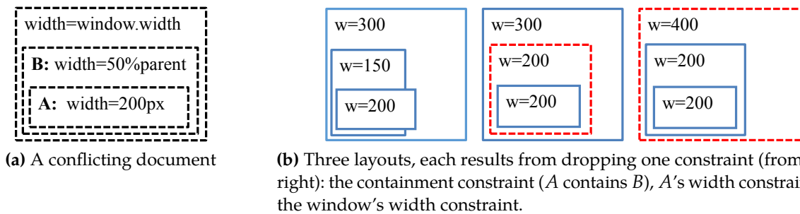
Figure 2.1.2. Dropping constraints leads to unpredictable layouts. When the window width is 300px, the document is conflicting (a). To display the document, solvers drop some constraints, creating many alternative ways to lay out the document. Three of which are shown (b).
