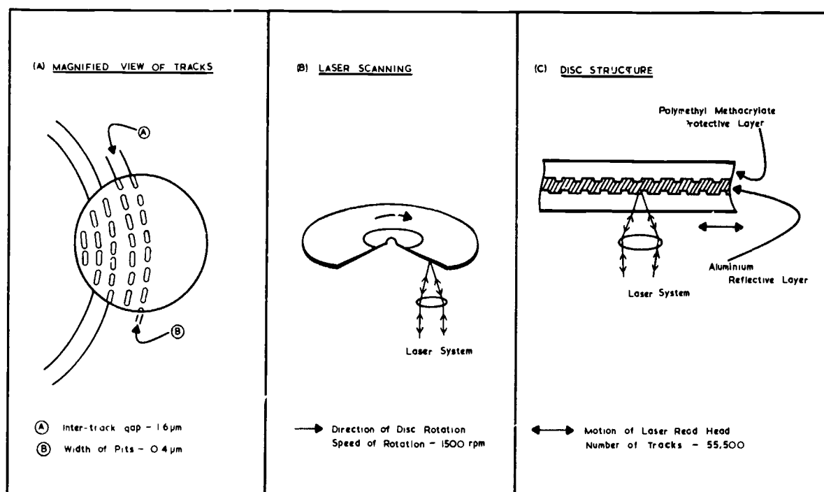
Fig 1 Structure and Mode of Operation of an Optical Disc
