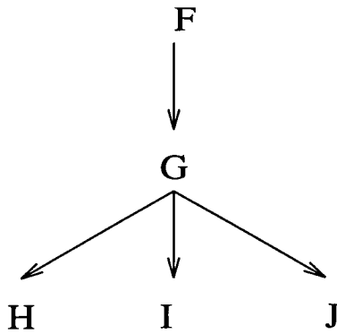
Figure 6.2: Example call-graph.
