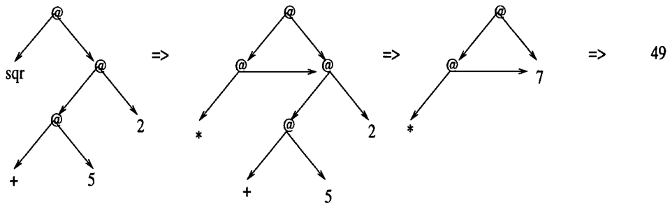
Figure 2.2: Graph reduction of \text{sqrt}(5 + 2) .
