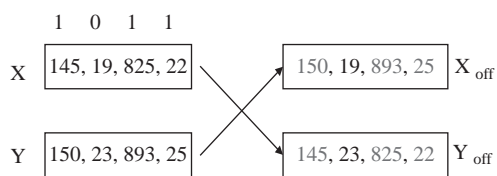
Fig. 3. An example of the crossover process.
