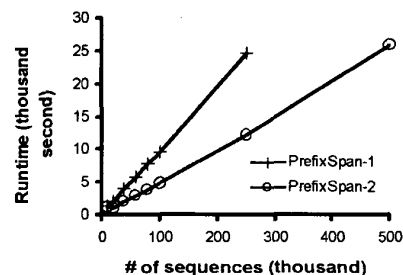
Figure 4. Scalability of PrefixSpan.
