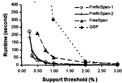
Figure 1. PrefixSpan, FreeSpan and GSP on data set C10T8S8I8 .
