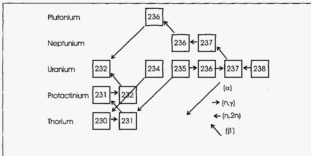
Figure 1. Reaction Chains Leading to the Production of ^{232}\text{U}
