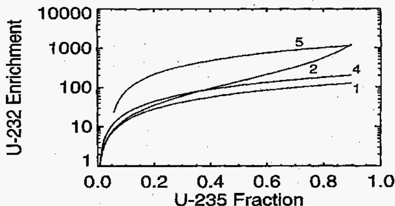
Figure 3. Four Estimates of the ^{232}\text{U} Enrichment as a Function of the ^{235}\text{U} Product Content Assuming a Depleted Tails Stream Containing 0.25% ^{235}\text{U}
