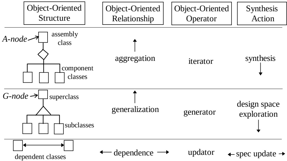
Fig. 1. Object-oriented structure, relationships, operators, and synthesis actions.
