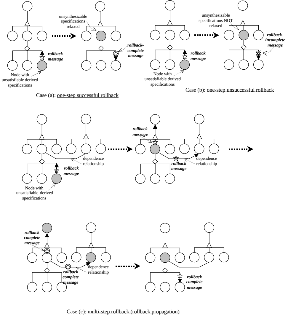
Fig. 10. Rollback process in POSE.
