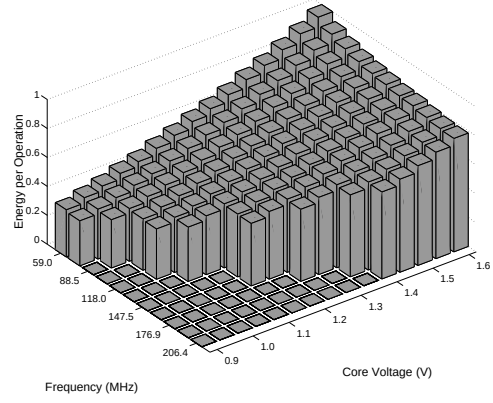
Figure 9: Measured energy consumption characteristics of SA-1100.
