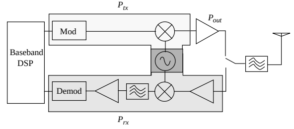
Figure 3: A diagram of the radio model.
