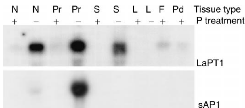
Fig. 2 Transcript abundance of phosphate ( P ) transporter (LaPT1) and secreted acid phosphatase (sAP1) in phosphate-sufficient and P-deficient white lupin at 14 d after emergence (DAE). Plants grown in presence of sufficient P are designated by (+) and those grown under P stress are designated by (-). Letters above each lane represent: N, normal roots; Pr, proteoid (cluster) roots; S, stems; L, leaves; F, flowers; Pd, pods. Flowers and pods did not form on -P plants. Each lane contains 20 \mu g of total RNA. (Derived from Liu et al. , 2001 and Miller et al. , 2001.)
