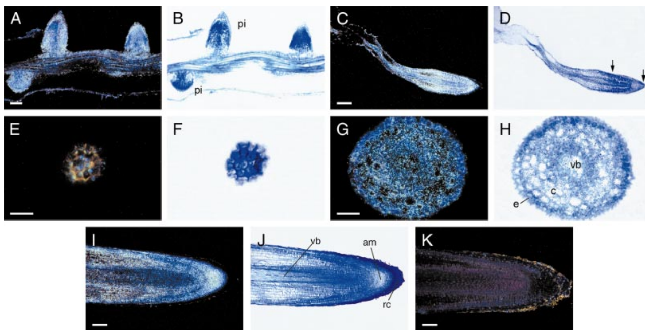
Fig. 5 In situ localization of phosphoenolpyruvate carboxylase (PEPC) in P-deficient cluster roots of white lupin. Sections A–J were hybridized with ^{35}\text{S} -labeled antisense RNA derived from LaPEPC1 cDNA, whereas section K was hybridized with the corresponding sense RNA probe. The dark-field (a, c, e, g, i and k) and bright-field (b, d, f and j) images correspond to longitudinal and transverse sections through cluster rootlets 9 d after emergence (DAE) (a, b) and 12 DAE (c–h) as well as through 12 DAE +P normal roots (i, j, k). Arrows in d indicate the approximate location of the two transverse sections shown in e–h. The areas that are white in a, c, e, g and i indicate the presence of PEPC mRNA. Sense control (K) showed no reaction. Bars are 50 \mu\text{m} (e, g), 100 \mu\text{m} (a) and 200 \mu\text{m} (c, i, k); pi, proteoid initials; vb, vascular bundle; c, cortex; e, epidermis, am, apical meristem, rc, rootcap. (Derived from Uhde-Stone et al. , 2003a.)
