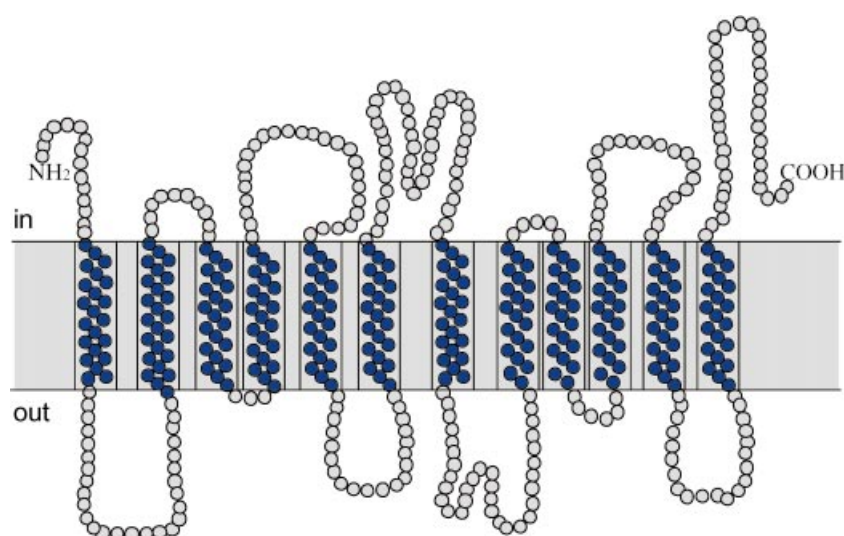
Fig. 1 Predicted topology of the high-affinity inorganic phosphate ( P_i ) transporter LaPT1 from white lupin based upon homology to other high-affinity P_i transporters.
