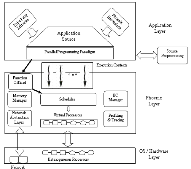
Figure 1. Phoenix ecosystem.
