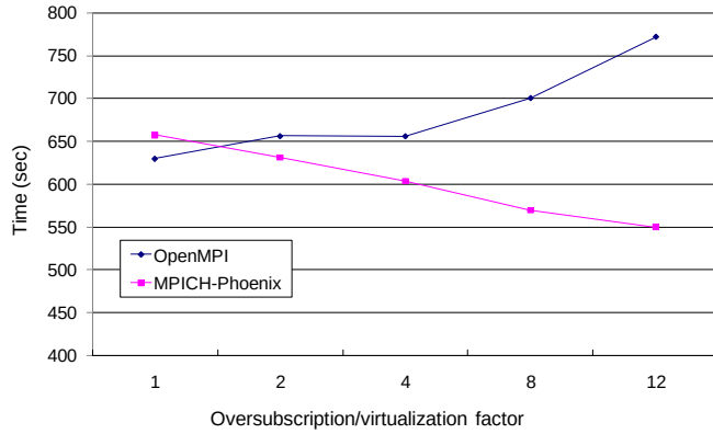
Figure 4. MILC runtime curves for OpenMPI and MPICH-Phoenix.
