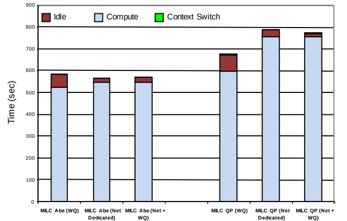
Figure 7. Integrated compute and communication scheduling for MILC.
