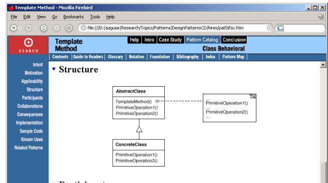
Figure 9. Template Method Pattern.
