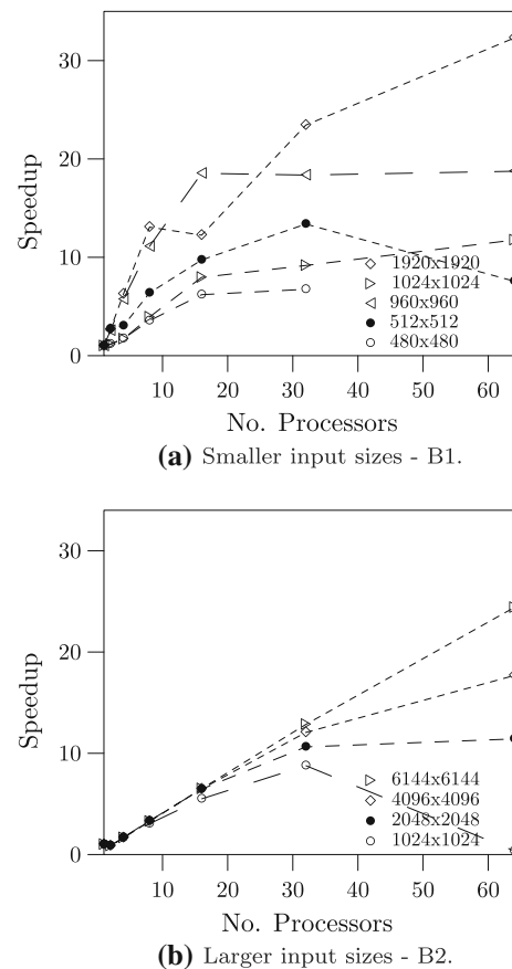
Fig. 4 Speedups for various input sizes
