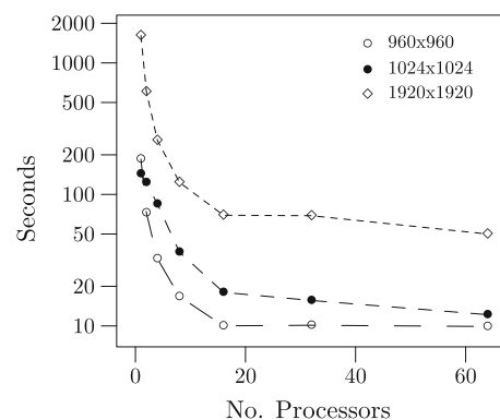
(b) Larger input sizes - B1.
