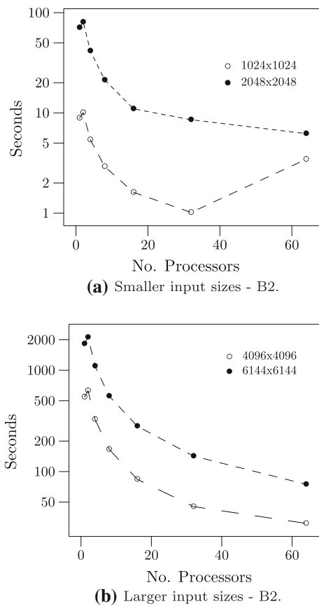
Fig. 3 Execution times for various input sizes—B2
