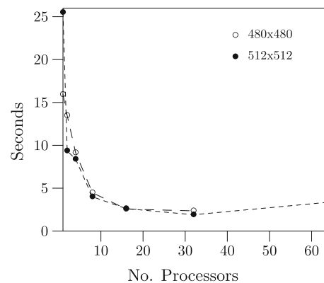
(a) Smaller input sizes - B1.
