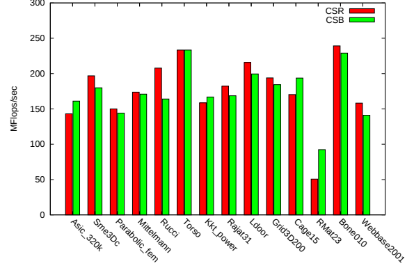
Figure 17: Serial performance comparison of SpMV for CSB and CSR.
