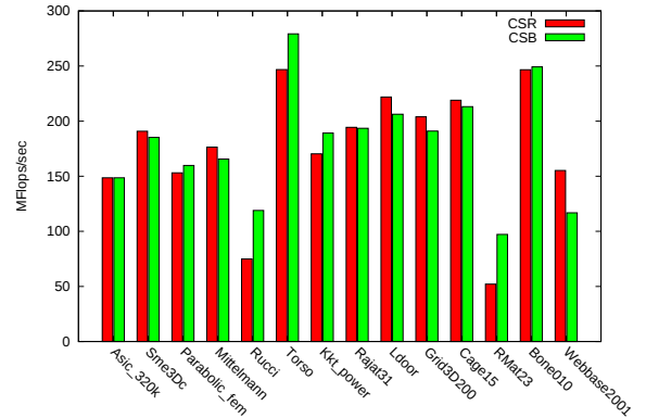
Figure 18: Serial performance comparison of SpMV_T for CSB and CSR.
