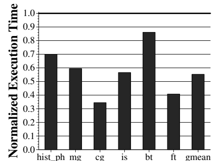
Figure 1: Potential execution time reduction if all inter-thread interference is ideally eliminated
