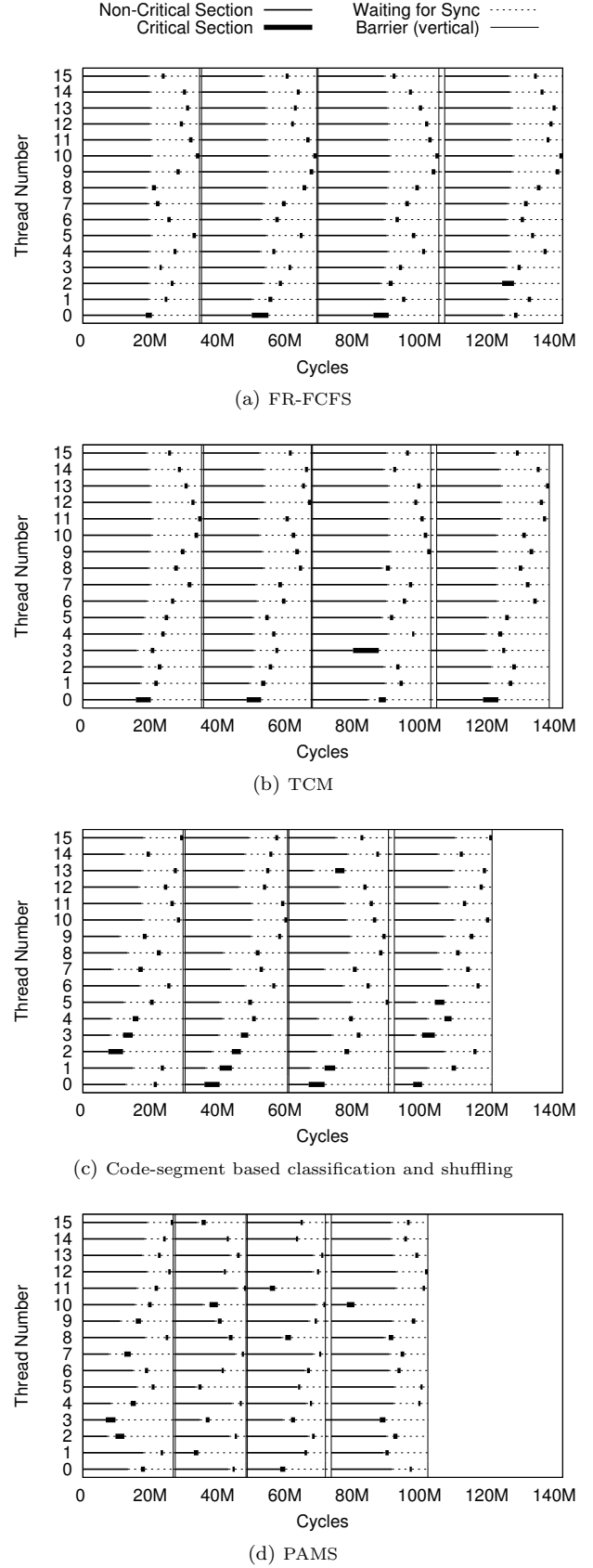
Figure 8: Execution of is benchmark with different memory scheduling techniques
