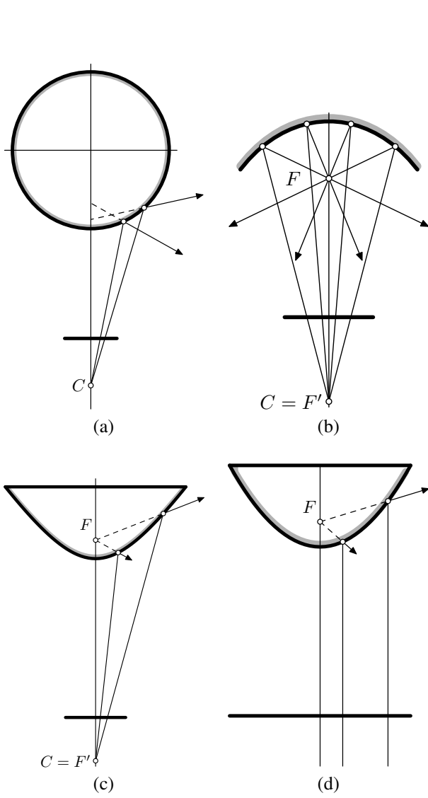
Figure 7: The combinations of a conventional central camera with (a) a spherical mirror (b), an elliptic mirror (c), a parabolic mirror (d), and a hyperbolic mirror. For elliptic (b) and hyperbolic (c) mirrors, there is a single viewpoint in F if the conventional camera center C is at F' . For parabolic mirrors (d), there is a single viewpoint in F if the mirror is imaged by an orthographic camera. There is no single viewpoint for a convex spherical mirror (a).
