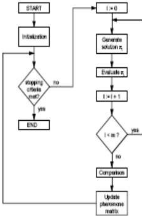
Fig. 3: ACO Processing Flow
