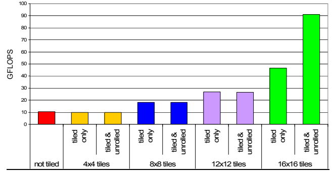
Figure 4. Performance of Matrix Multiplication Kernels
