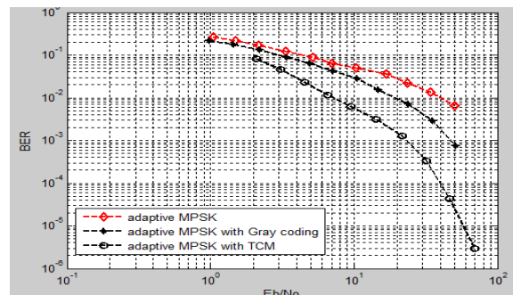
Fig.4. BER vs E_b/N_0 graph for Adaptive MPSK . adaptive MPSK with gray coding and adaptive MPSK with TCM for MIMO-OFDM system under flat fading channel.
