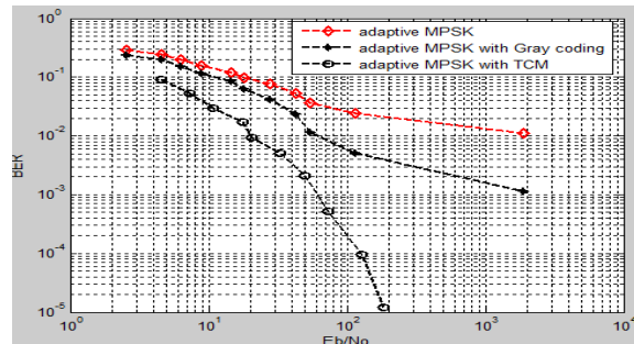
Fig.3. BER vs E_b/N_0 values for adaptive MPSK, adaptive MPSK with Gray coding and adaptive MPSK with TCM SISO-OFDM system under flat fading channel.
