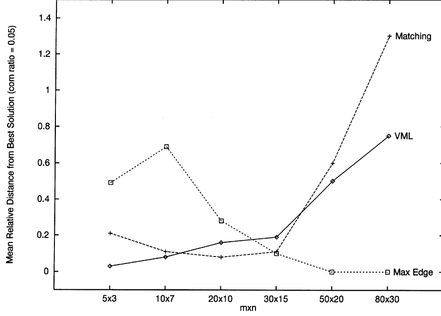
FIG. 5. Mean relative distance com ratio 0.05. Critical point is 30 \times 15 .
