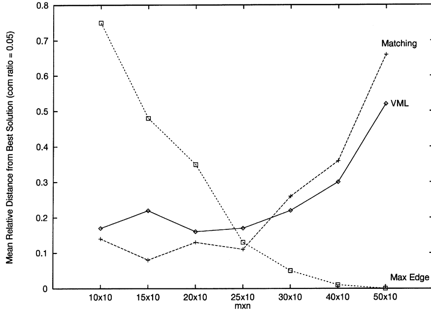
FIG. 6. Mean relative distance for com ratio 0.05 and for 10 processors.
