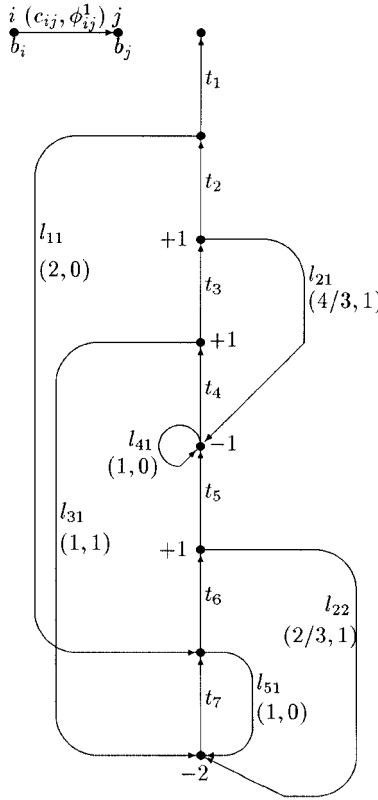
FIG. 3. Sample flow problem solved by \mathcal{W} .
