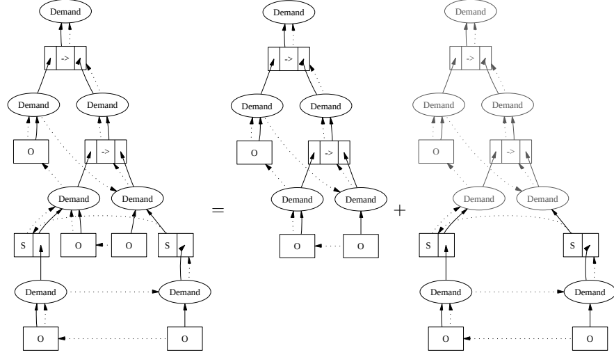
Fig. 4. Separating the extended COOSy trace of Example 9
