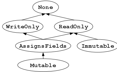
Figure 15. The type hierarchy for immutability parameters of Fig. 6 extended with WriteOnly and None .
