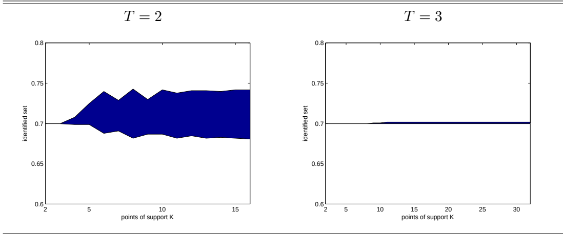
Figure 1: Identified sets in a simple static logit model with time trend
