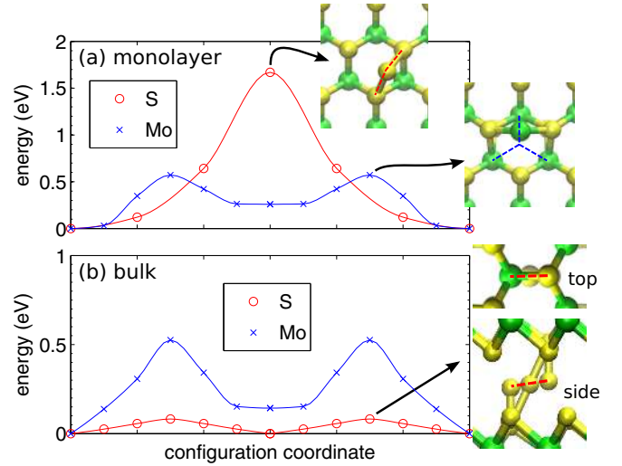
FIG. 12. (Color online) Energy along the migration path for diffusion of (a) adatoms on the monolayer surface and (b) interstitials inside bulk. Insets of (a) illustrate the saddle-point configurations for Mo and S migration paths on monolayer. Dashed lines illustrate the whole path. Insets of (b) show the saddle-point configuration and migration path for S interstitial. The path for Mo is similar to that in (a), but starting from the center of hexagon.
