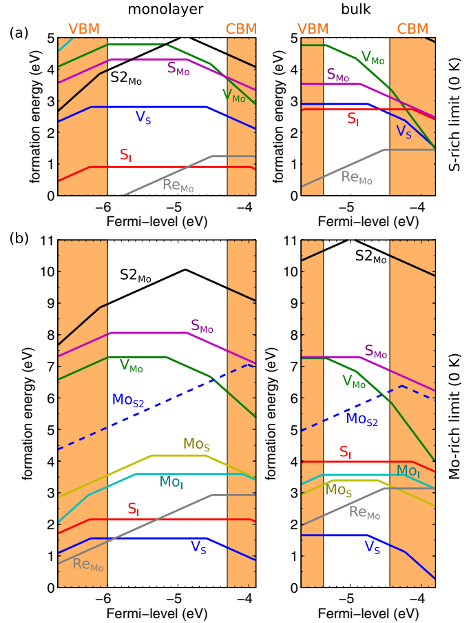
FIG. 7. (Color online) Formation energies as a function of the Fermi-level position calculated with the PBE-D functional for monolayer (left) and bulk (right) in the S-rich (top, \mu_S = 0 eV) and Mo-rich (bottom, \mu_S = -1.25 eV) chemical potentials, corresponding to 0 K. The coloring of the lines is the same as in Fig. 6. PBE-D calculated band edge positions are also shown. The energy zero of the Fermi level in both cases is at vacuum.
