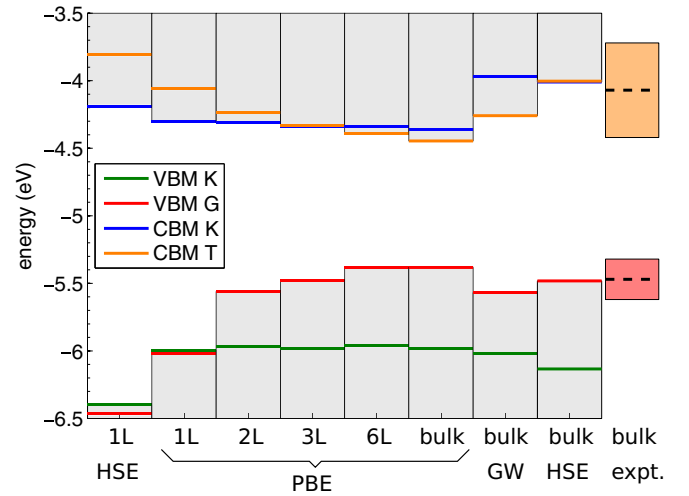
FIG. 4. (Color online) Valence and conduction band edge positions with respect to vacuum level as calculated using different levels of theory and different number of MoS 2 layers. The highest energy valleys of the valence band are located at K and \Gamma , and the lowest energy valleys of the conduction band at K and T (about half-way between \Gamma and K ). Experimental values are from Ref. [118].
