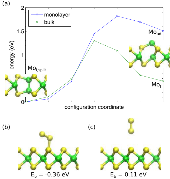
FIG. 13. (Color online) (a) Energy barrier for the Mo migration from the adatom or interstitial site to the \text{Mo}_{\text{I,split}} configuration. The energy of \text{Mo}_{\text{I,split}} is set to zero both in bulk and in monolayer. (b),(c) Visualization of the two (meta-)stable configurations for \text{S}_2 molecule on top of \text{MoS}_2 and the binding energy E_b = E(\text{MoS}_2) + E(\text{S}_2) - E(\text{MoS}_2 + \text{S}_2) (a positive value corresponds to binding to the surface).
