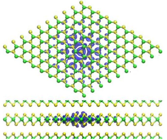
FIG. 9. (Color online) Top and side view of partial charge density isosurface from the wave function of the Re substitutional defect in the Mo site in 2H-MoS 2 .
