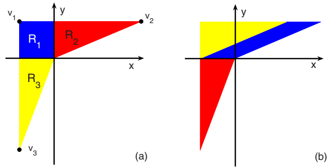
FIG. 3. (Color online) (a) For \mu < 0 , partition of B into three regions: R_1 (blue), R_2 (red), and R_3 (yellow). Black filled dots indicate the points v_1, v_2 , and v_3 , respectively. (b) First iterations of the respective regions in (a) under the map F .
