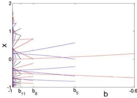
FIG. 1. (Color online) Bifurcation diagram of Eq. (1) for a=-2 showing the occurrence of multiple coexisting periodic attractors. At each bifurcation point b_i , a new periodic attractor of period i appears. In fact, the period of any newly appeared attractor is increased arithmetically. The precise values of various b_i are given in Table I.
