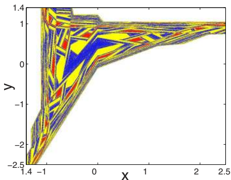
FIG. 2. (Color online) For a=-2 and b=-0.95 in Eq. (1), basins of attraction of three distinct periodic attractors and an additional attractor at infinity. Blank regions indicate the initial conditions that lead to trajectories approaching infinity. The blue, yellow, and red regions denote the basins of the periodic attractors of period 2, 5, and 8, respectively.
