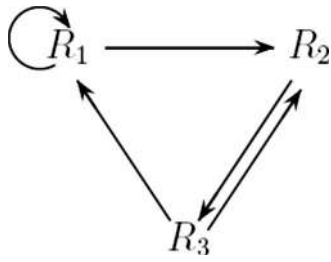
FIG. 4. Transition graph characterizing the dynamics on the invariant set B_\mu under Eq. (1).
