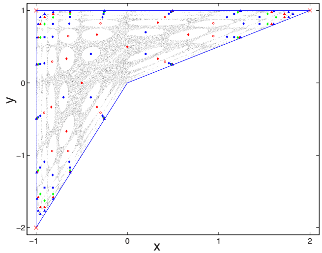
FIG. 5. (Color online) For Eq. (1) in the Hamiltonian limit ( \mu = -1 ), chaotic sea, elliptic periodic orbits, and KAM island chains. Blue lines indicate the boundary of the invariant set and markers indicate elliptic periodic orbits in the KAM islands: red crosses for an unstable period-3 orbit, red filled circles for a period-2 orbit, blue filled circles for a period-5 orbit, red filled diamond for a period-8 orbit, red circles for a period-11 orbit, blue filled diamond for a period-14 orbit, blue filled rectangles for a period-17 orbit, green filled diamond for a period-20 orbit, red filled triangles for a period-23 orbit, and blue filled triangles for a period-26 orbit.
