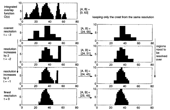
Fig. 5. Overlap function \Omega(x) and its appearance at different resolutions. (The shaded region indicates the region needs to be resolved over.)
