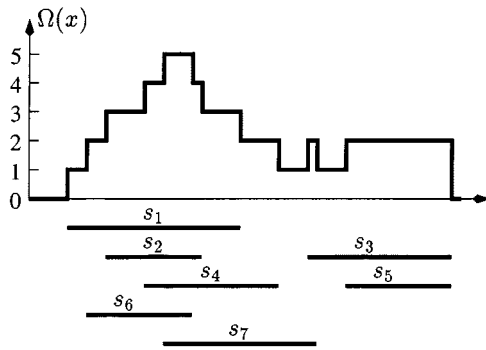
Fig. 4. Overlap function for a set of seven sensors.
