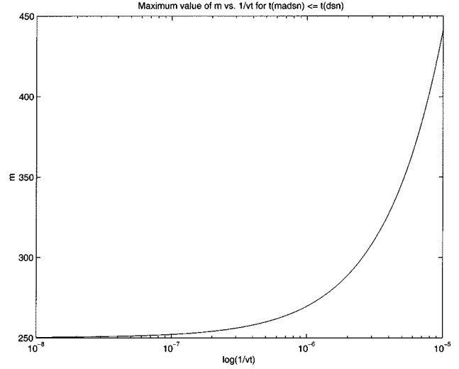
Fig. 10. Performance evaluation between DSN and MADSN: m vs. 1/v_n .
