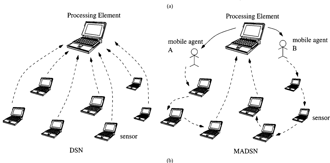
Fig. 1. Comparison between DSN and MADSN. (a) Feature. (b) Architecture.
