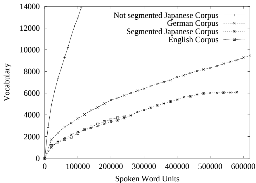
Figure 1. Vocabulary growth comparing German, English and Japanese
